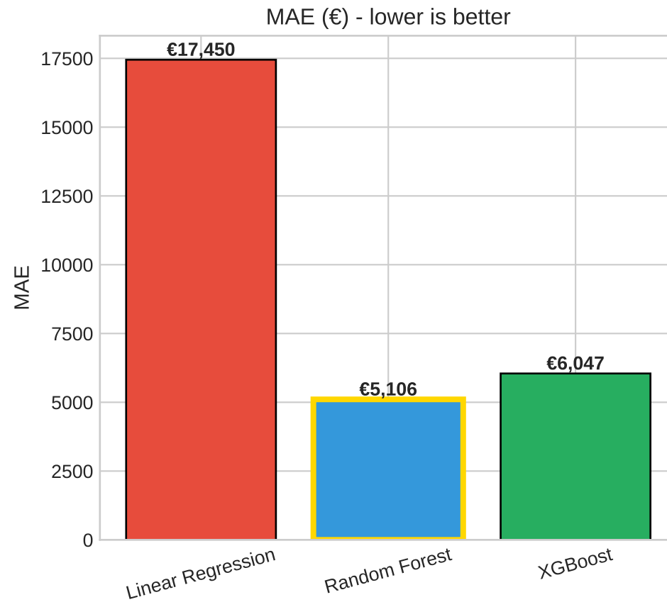
Figure 7b: Final Model Performance Comparison
